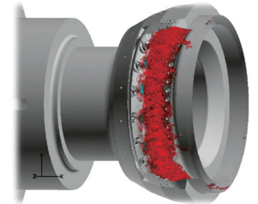
Large-eddy simulation of turbulent spray combustion field of full annular combustor for aircraft engine (In Proc. of GTC2015)
