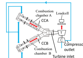
Gas Turbine with a Pulse Combustor
