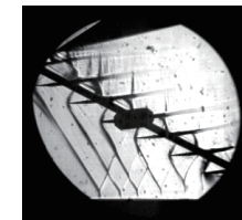
Transonic Cascade Flow
