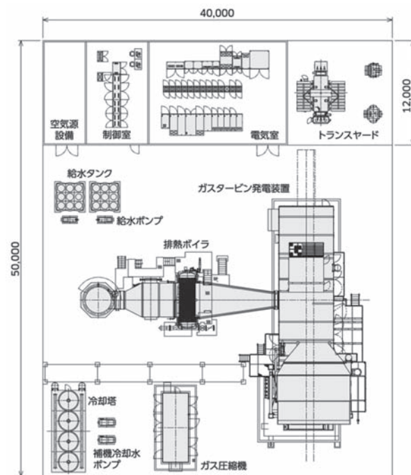
Fig.15 PUC300D arrangement
