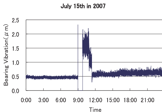
Fig. 4 Vibration of waterwheel on 15th of July in 2007
