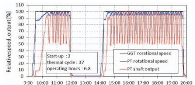
Fig. 4 Typical operating pattern during cyclic testing
