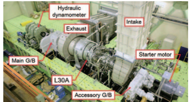
Fig. 3 Engine testing facility
