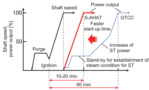
Fig.11 Concept of hot start-up of the S-AHAT
