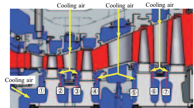
Fig. 7 Cooling of turbine rotor outer circumference
