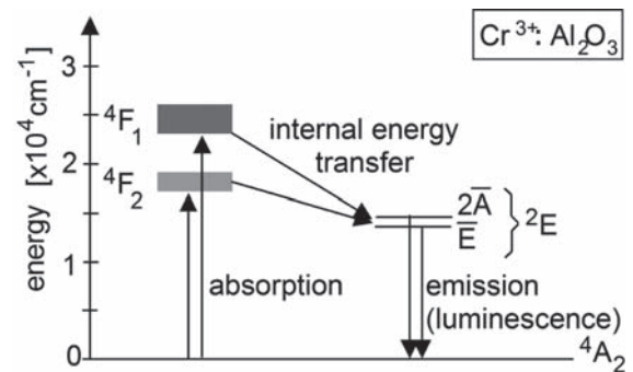
Fig.10 Energy level diagram of Cr 3+ in Al 2 O 3
