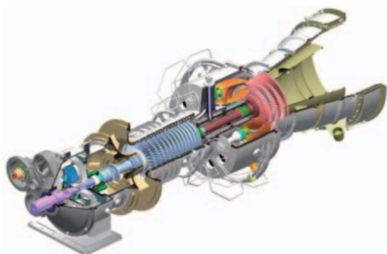
Fig. 7 Taurus 65 Gas Turbine
