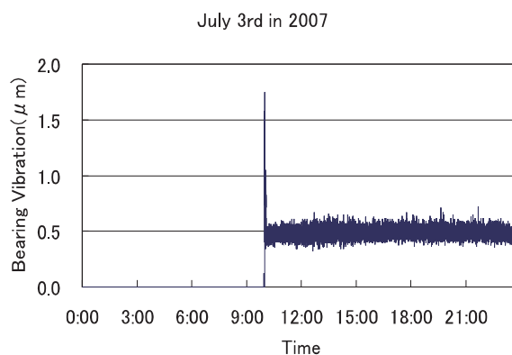
Fig. 5 Vibration of waterwheel on 3rd of July in 2007
