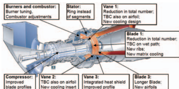
Fig. 6 Main design modification from 47.5MW to 50.5MW
