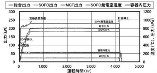
Fig. 10 Long term behavior of model 10 SOFC-MGT hybrid system installed at Tokyo Gas Co.,Ltd.'s Senju Techno Station (It was provided by MHPS)
