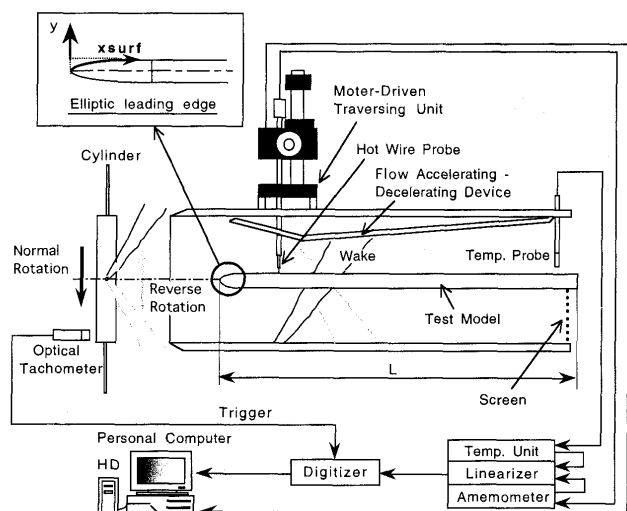
図2 Test model and measurement system
