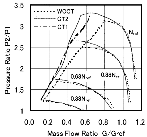
Fig.4 Improvement of surge limit by casing treatment
