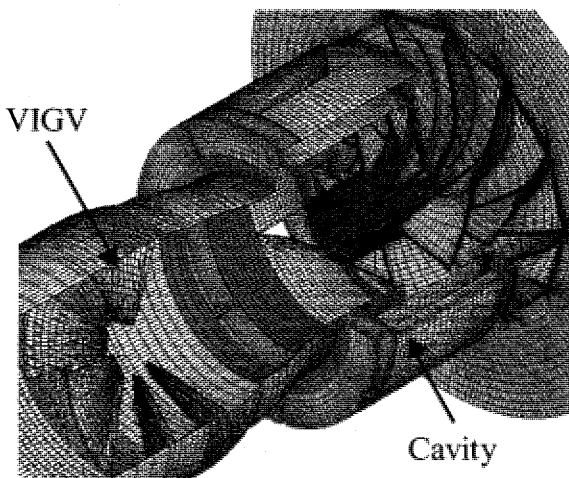
Fig.3 Computing grid
