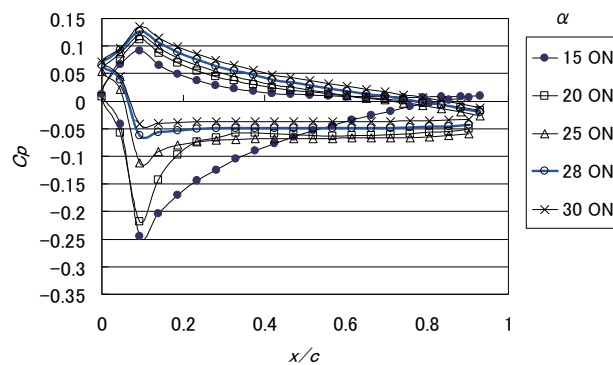
Fig.13 C_p distributions for various angles of attack ( U = 70 m/s, Plasma ON, f = 900 Hz)
