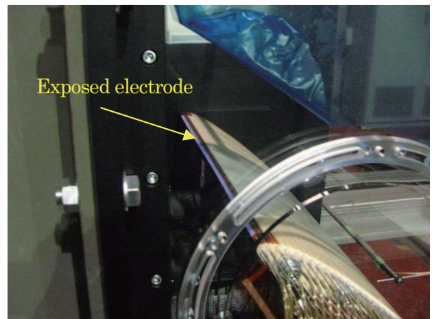
Fig. 4 Operating plasma actuator electrode
