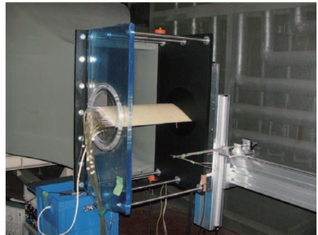
Fig. 2 Model NACA0015 wing with wind tunnel
