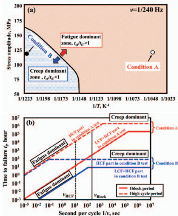
Fig. 14 Failure mode prediction curve (a) at cyclic frequency v = 1/240 \text{ Hz} (1block), and (b) relationship between time to failure and cyclic frequency under conditions A and B.
