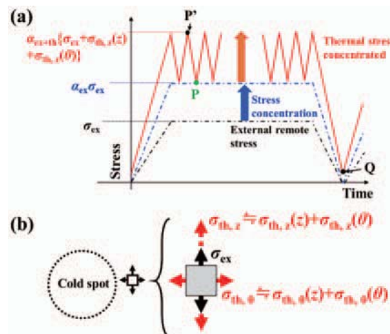
Fig. 4 (a) Schematic diagram on local thermal stress under the Condition A when thermal stress is superimposed on mechanical stress and (b) remote thermal stress near the cold spot at point P'.
