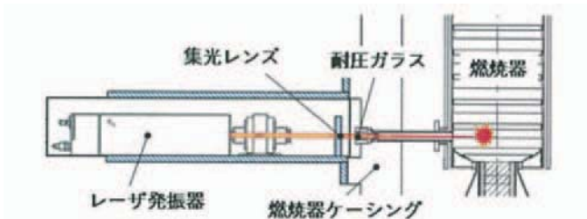
Fig. 11 Laser Ignition for CO 2 Turbine (12)
