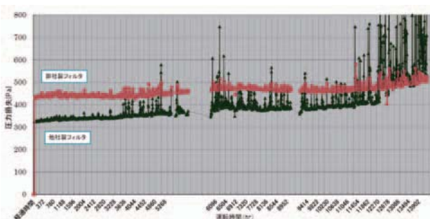
Fig. 6 Sample comparison trend curve of HEPA filter by Shinwa and other Supplier
