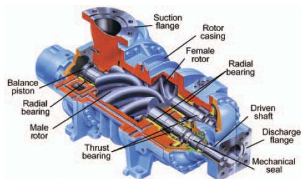
Fig. 4 Compressor cutaway
