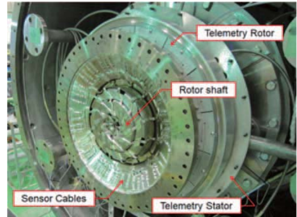
Fig. 3 Telemetry system
