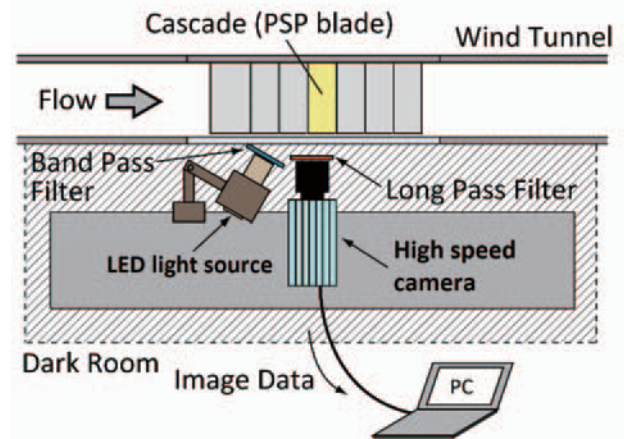
Fig. 2 PSP measurement system (3)
