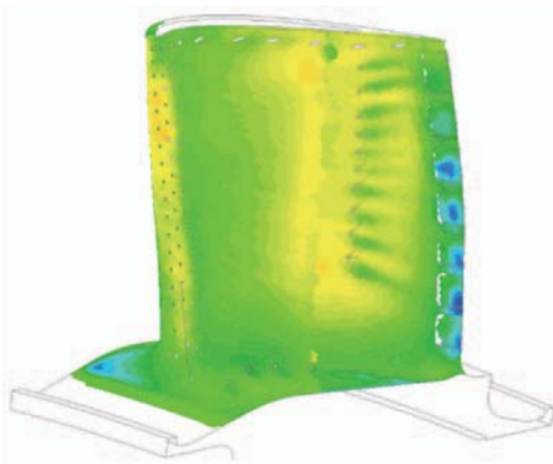
Fig. 15 Pyrometer measurement result
