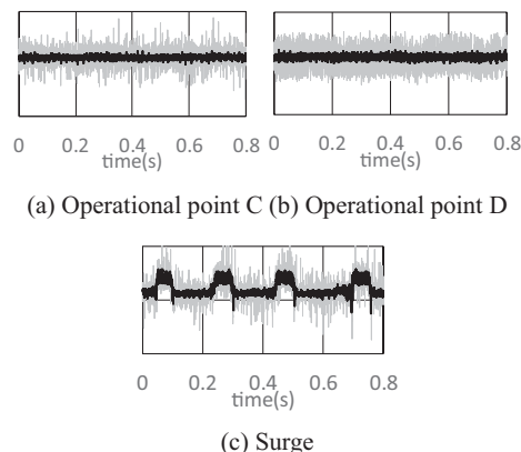
Fig. 17 Signal from pressure transducer at v
