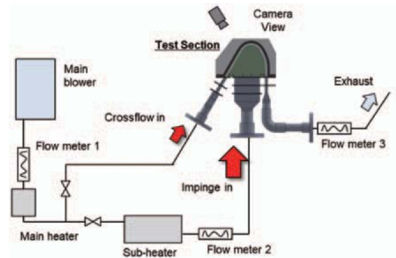
Fig. 6 Experimental system for internal cooling
