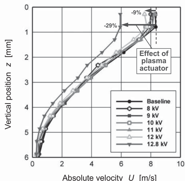
Fig. 5 Absolute velocity distributions near tip clearance exit of flat plate at various DBD-PA input voltages ( f_p = 8.6 kHz) at x = 28.6 mm
