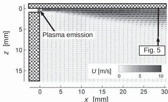
(c) Flow control ( V_{p-p} = 12.8 kV, f_p = 8.6 kHz)
