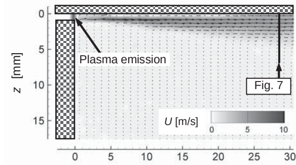
(c) Flow control ( f_p = 10 kHz)
