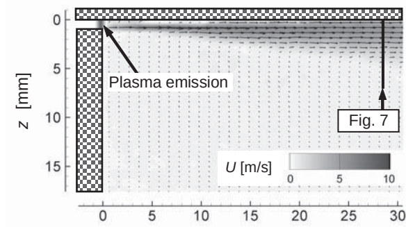
(b) Flow control ( f_p = 8.6 kHz)
