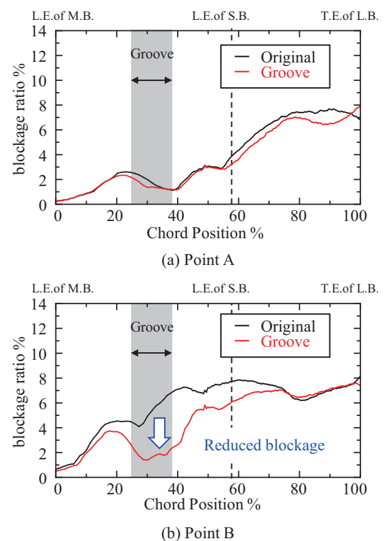
Fig. 7 Blockage Ratio Distribution in Original and Groove.
