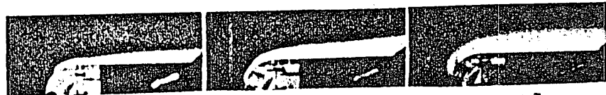
図9. 煙吹出実験 (模型I, Re_\infty = 1.5 \times 10^4 )
